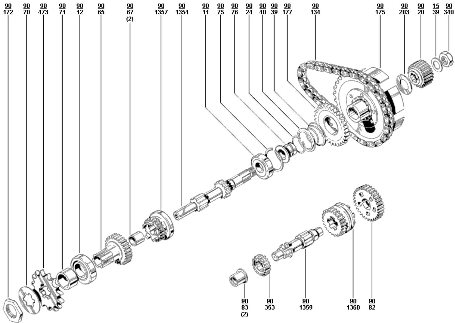
GEARBOX AND FITTINGS
