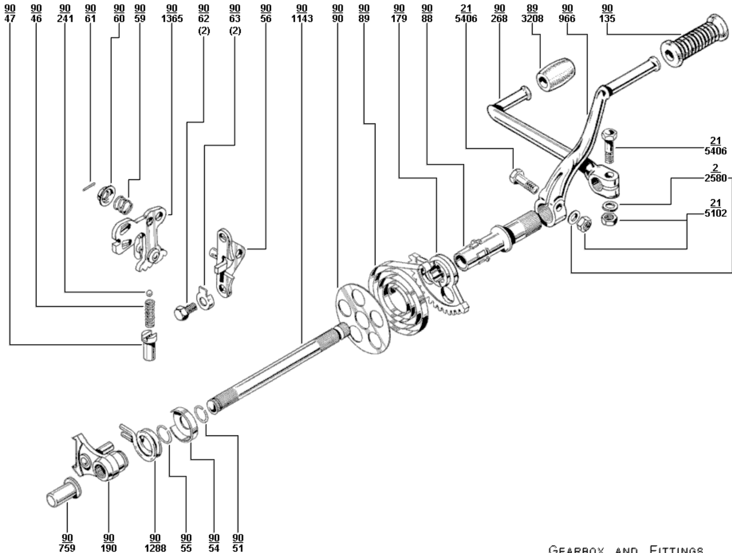
GEARBOX AND FITTINGS
