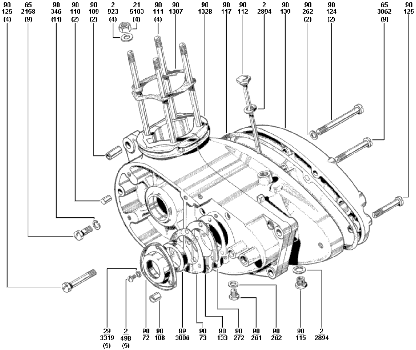
ENGINE AND GEARBOX
